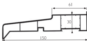
150mm Deep Nosed cill
