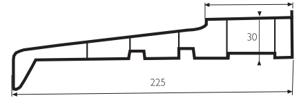
225mm Deep Nosed cill
