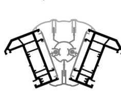
Window Widgets variable post
