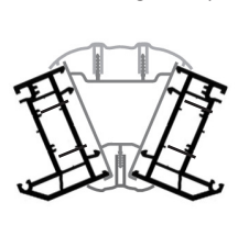
Window Widgets 135 degree post (Also available in 150)
