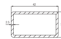
Reinforcement* 42 x 23 x 2.5mm Art. No. 261738
