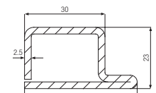
Reinforcement 42 x 30 x 23 x 2.5mm Art. No. 200347
