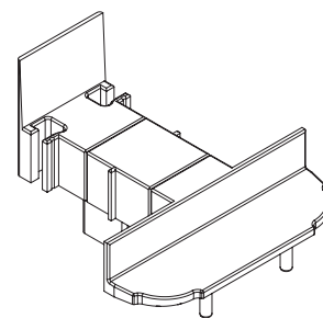
Art. No. 286928 Dummy Mullion Endcap for Sculptured Suite To Fit Art. No. 546660 Slim 'T' Transom
