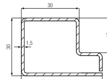
Reinforcement 42 x 30 x 30 x 18 x 1.5mm Art. No. 200327
