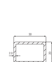
Reinforcement 30 x 20 x 2mm Art. No. 255924
