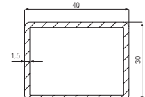
Reinforcement 40 x 30 x 1.5mm Art. No. 258358
