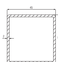
Reinforcement* 45 x 45 x 2mm Art. No. 259894
