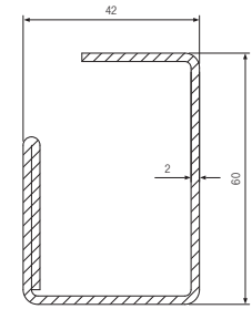
Reinforcement 42 x 60 x 2mm Art. No. 287066
