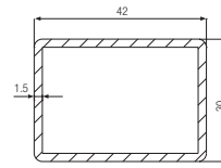
Reinforcement* 42 x 30 x 1.5mm Art. No. 261958
