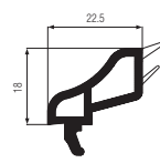
Glazing Bead 22.5mm White Art. No. 551510 Laminated Art. No. 581580
