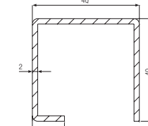
Reinforcement* 40 x 40 x 40 x 12 x 2mm Art. No. 252827
