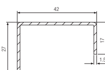
Reinforcement 42 x 27 x 17 x 1.5mm Art. No. 264434
