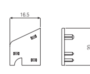
End Cap for Weather Rail Art. No. 269460/002 Right - White Art. No. 269470/002 Left - White Art. No. 269460/003 Right - Brown Art. No. 269470/003 Left - Brown
