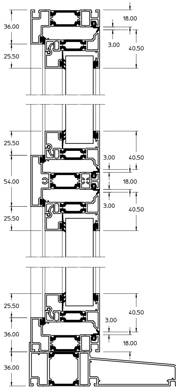
External Flush
