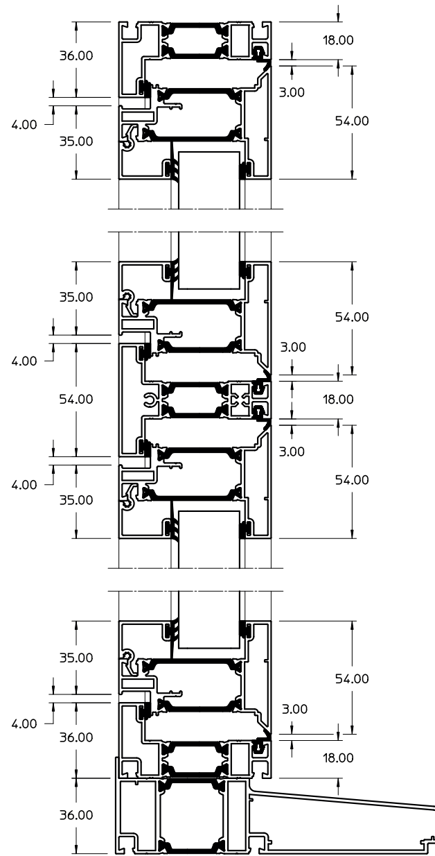
Fully Flush
