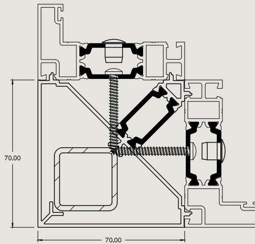
90 degree Baypole
