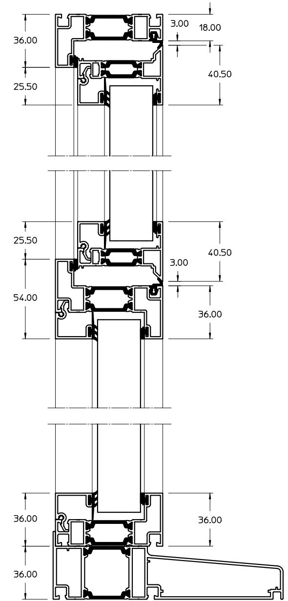
Reversed Butt
