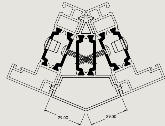
135 degree Baypole
