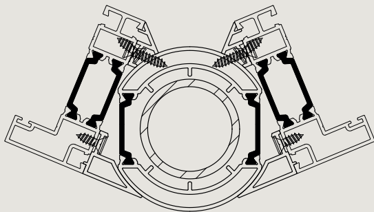
Variable Baypole
